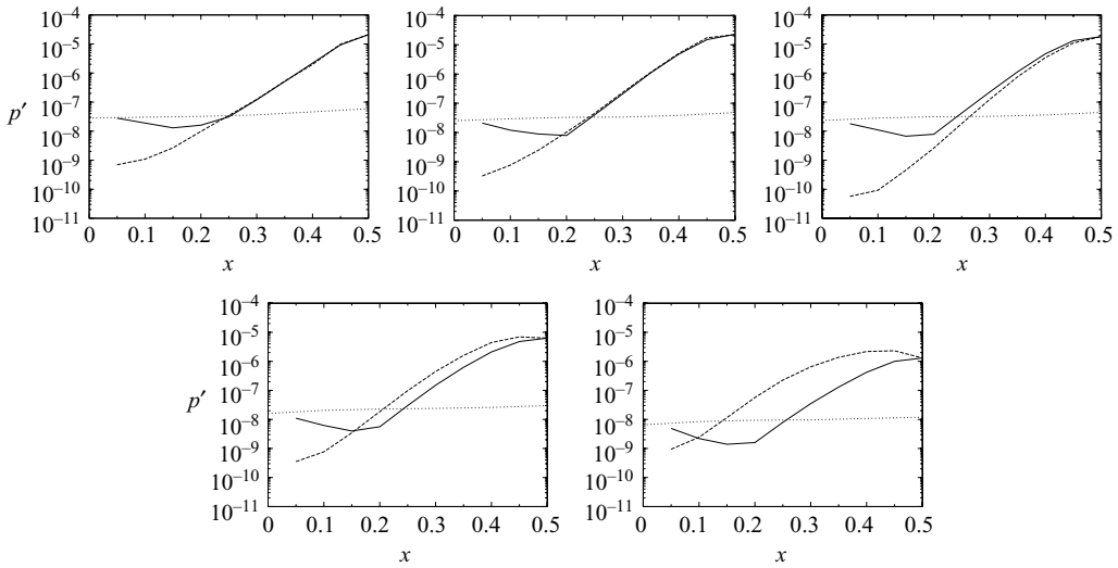
FIGURE 32. Amplitude of pressure fluctuations as a function of x , recorded at locations within the aerofoil boundary layer (—), outside the aerofoil boundary layer ( \cdots ) and the equivalent instability growth curve as computed via DNS (---). From left to right, the top row shows f = 6.1 , f = 8.49 and f = 9.15 , and the bottom row shows f = 11.2 and f = 14.25 .
