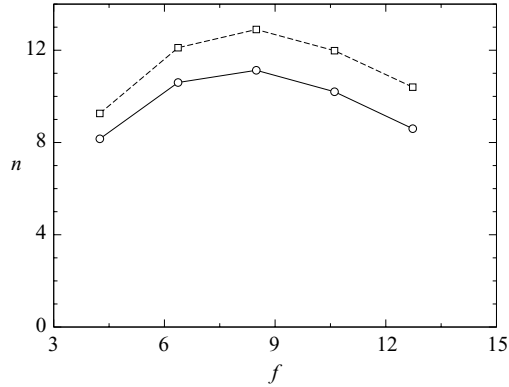
FIGURE 13. Variation of the maximum N -factor with frequency, showing DNS results ( \circ - \circ ) and LST predictions ( \square - \square ).
