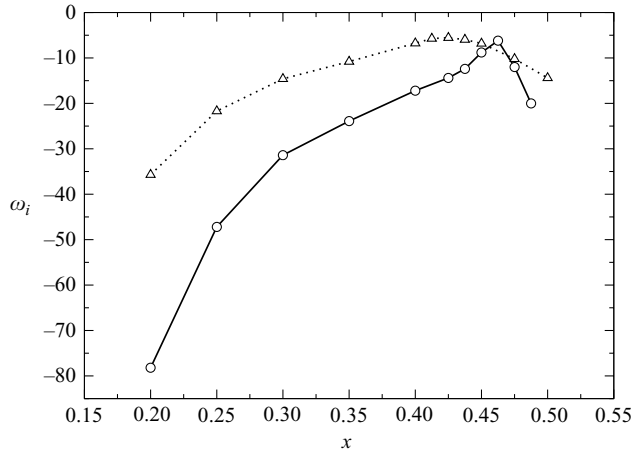
FIGURE 14. Variation with x of \omega_i associated with c_g = 0 , for the reference flow from the two-dimensional case ( \circ - \circ ) and the reference flow from the three-dimensional case ( \triangle \cdots \triangle ) at \alpha = 5^\circ .
